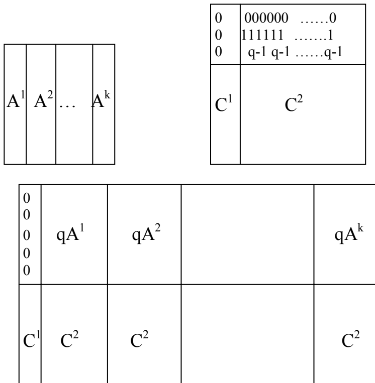
Figure 12. Construction for Theorem 7.1.
