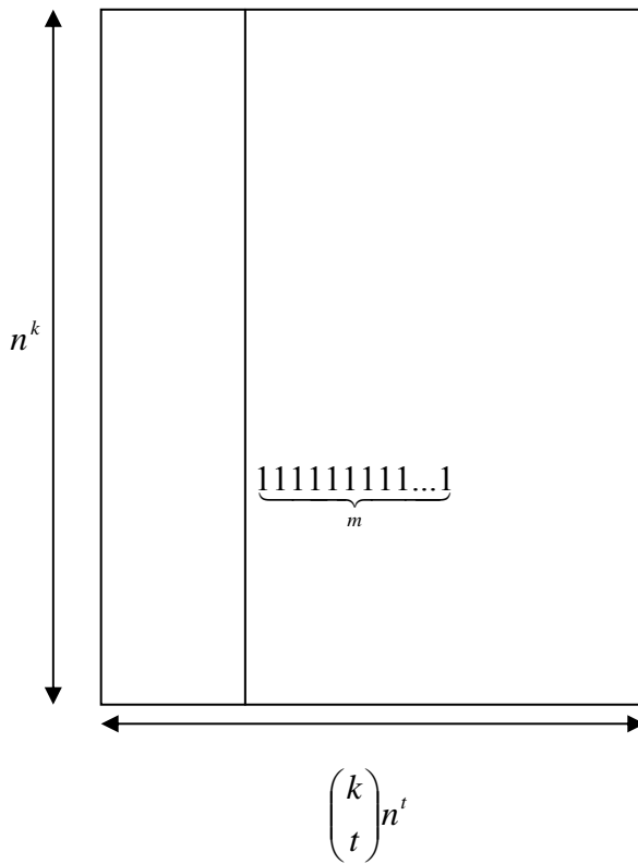
Figure 10. Proof of Equation (1).
